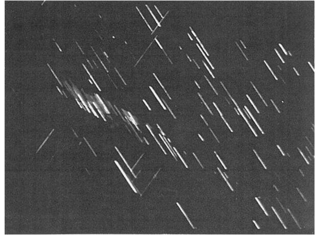
Figure 6 Typical DF micrograph of S' precipitates. Magnification \times 38000 .
