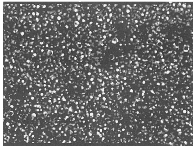
Figure 2 DF micrograph of homogeneously distributed \delta' precipitates of B alloy in under-aged condition. Magnification \times 38000 .
